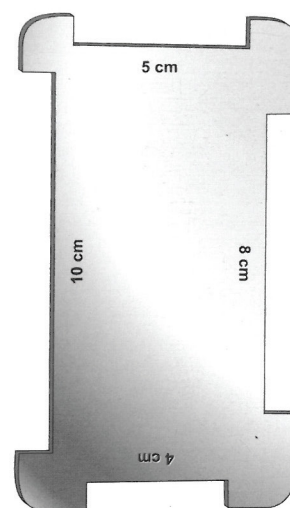
Schink V10-0120 Skin straightening plate only
